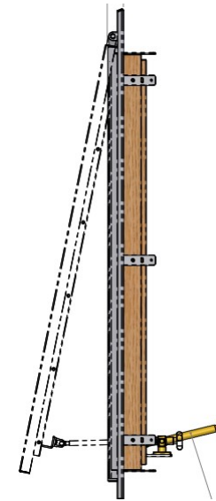
SECTION A-A Opening Roof Window
