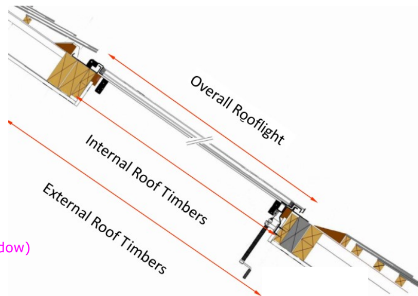
SECTION A-A Opening Roof Window
